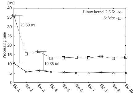
Fig. 4. Processing times of the open() system call
