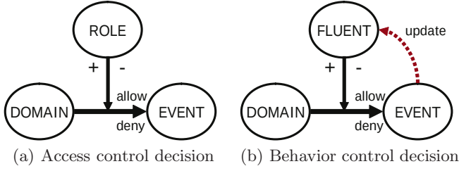
Fig. 2. Security decisions
