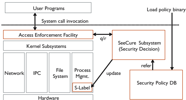
Fig. 3. System architecture
